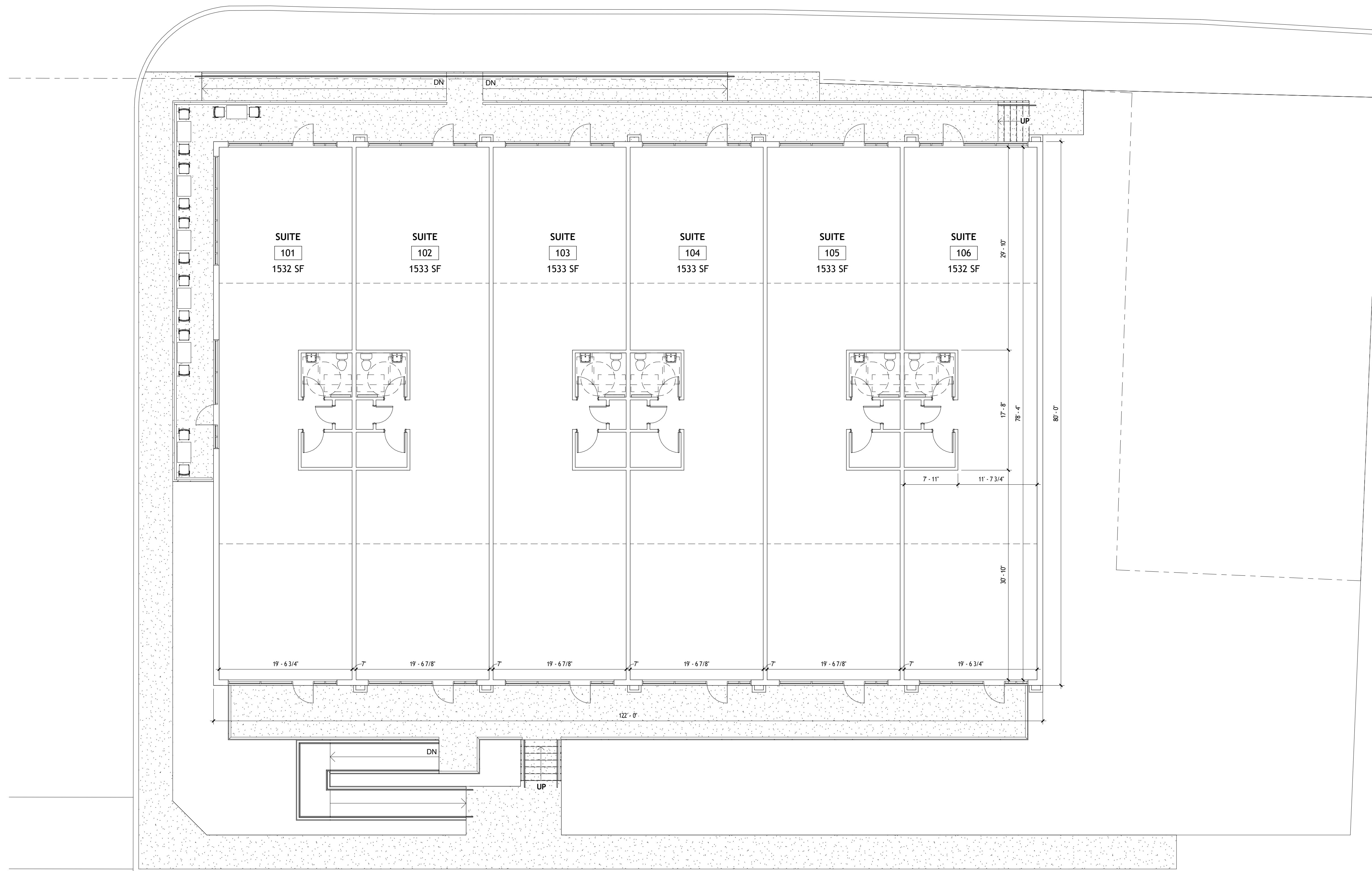
1 PRELIMINARY FLOOR PLAN SCALE: 1/8" = 1'-0"
